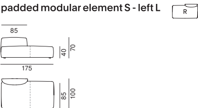
padded modular element S - left L
