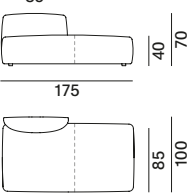
padded modular element L - left L
