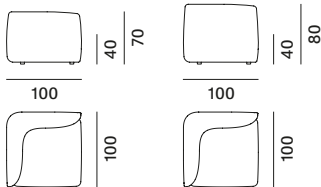
padded corner modular elements
