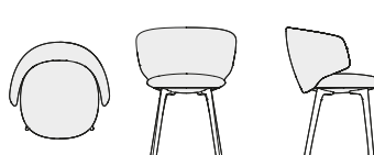
4-legged oak base L59 D57 H78 seat H51
